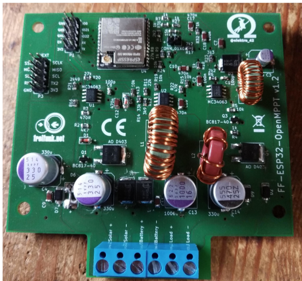
Figure 2: OpenMPPT circuit board
